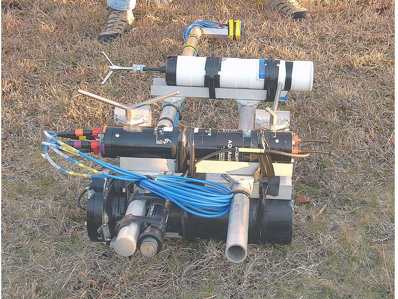
Figure 5. Pole mount for the acoustic Doppler velocimeter Triton, acoustic backscatter sensor, and associated pressure cases. Photograph by Don Bowers.
